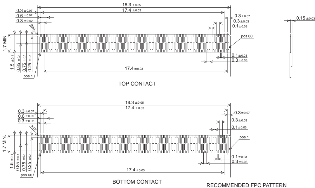
RECOMMENDED FPC PATTERN
