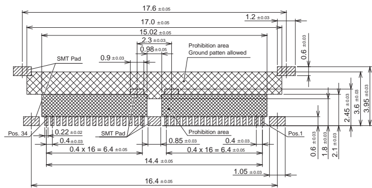
RECOMMENDED FOOTPRINT PATTERN
